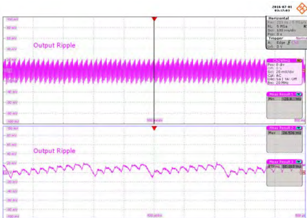
Figure 44 – 85 VAC Input. Condition: 18 V – 250 mA, 5 V – 50 mA. V_{RIPPLE} , 20 mV / div., 100 ms, 100 \mu s / div.
