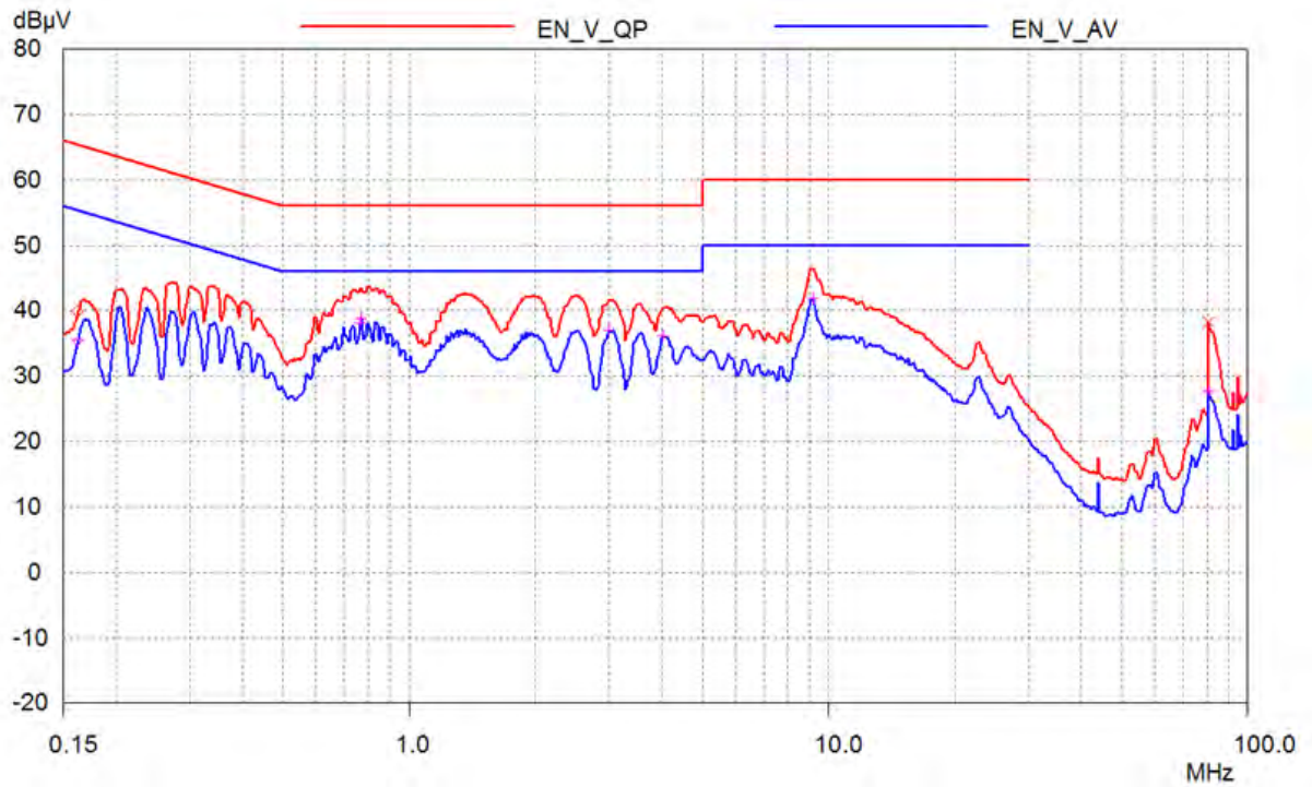
Figure 50 – Floating Negative Output at 230 VAC, Neutral.
