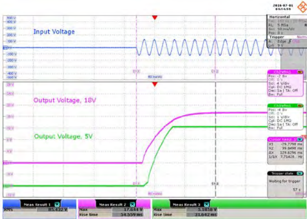
Figure 34 – 85 VAC Input. Condition: 18 V – 250 mA, 5 V – 50 mA. Upper: V_{IN} , 100 V, 50 ms / div. Middle: V_{OUT1} , 4 V / div. Lower: V_{OUT2} , 1 V / div.
