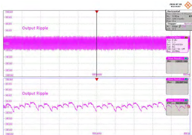
Figure 45 – 265 VAC Input. Condition: 18 V – 250 mA, 5 V – 50 mA. V_{RIPPLE} , 20 mV / div., 100 ms, 100 \mu s / div.
