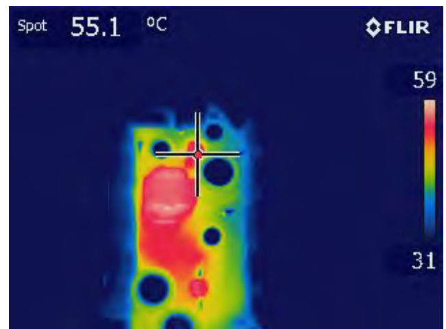
U2 – Linear Regulator. Spot Temperature – 55.1 °C.
