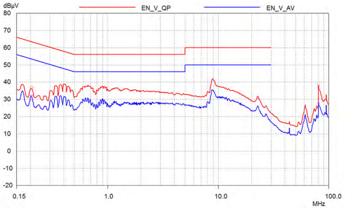
Figure 48 – Floating Negative Output at 115 VAC, Neutral.
