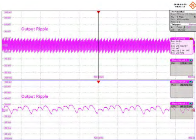
Figure 42 – 85 VAC Input. Condition: 18 V – 250 mA, 5 V – 0 A. V_{RIPPLE} , 20 mV / div., 100 ms, 100 \mu s / div.
