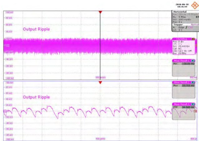
Figure 43 – 265 VAC Input. Condition: 18 V – 250 mA, 5 V – 0 A. V_{RIPPLE} , 20 mV / div., 100 ms, 100 \mu s / div.
