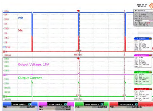
Figure 37 – 265 VAC Input. Condition: 18 V – Shorted, 5 V – 50 mA. Auto-Restart: 1.49 s. Upper: V_{DS} , 50 V / div., 500 ms / div. Upper Middle: I_{DS} , 500 mA / div. Lower Middle: V_{OUT18} , 4 V / div. Lower: I_{OUT18} , 400 mA / div.
