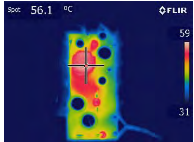
T1 – Transformer. Spot Temperature – 56.1 °C.
