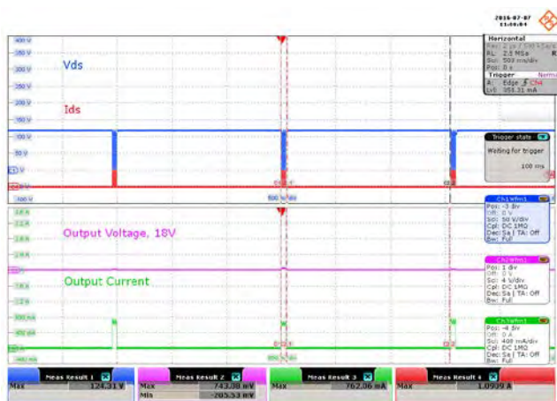
Figure 36 – 85 VAC Input. Condition: 18 V – Shorted, 5 V – 50 mA. Auto-Restart: 1.49 s. Upper: V_{DS} , 50 V / div., 500 ms / div. Upper Middle: I_{DS} , 500 mA / div. Lower Middle: V_{OUT18} , 4 V / div. Lower: I_{OUT18} , 400 mA / div.
